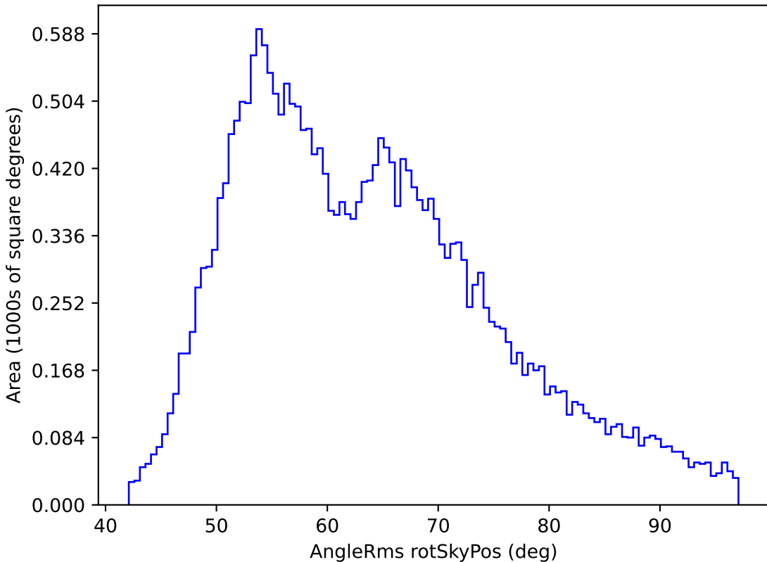
too_100_1v3.4_10yrs All sky r band: AngleRms rotSkyPos
