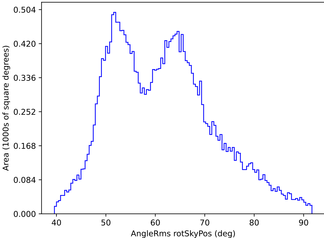
too_100_1v3.4_10yrs All sky i band: AngleRms rotSkyPos
