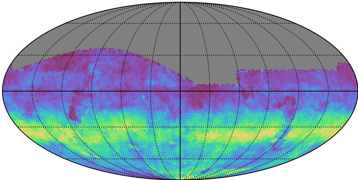
too_100_1v3.4_10yrs All sky g band: AngleRms rotSkyPos
