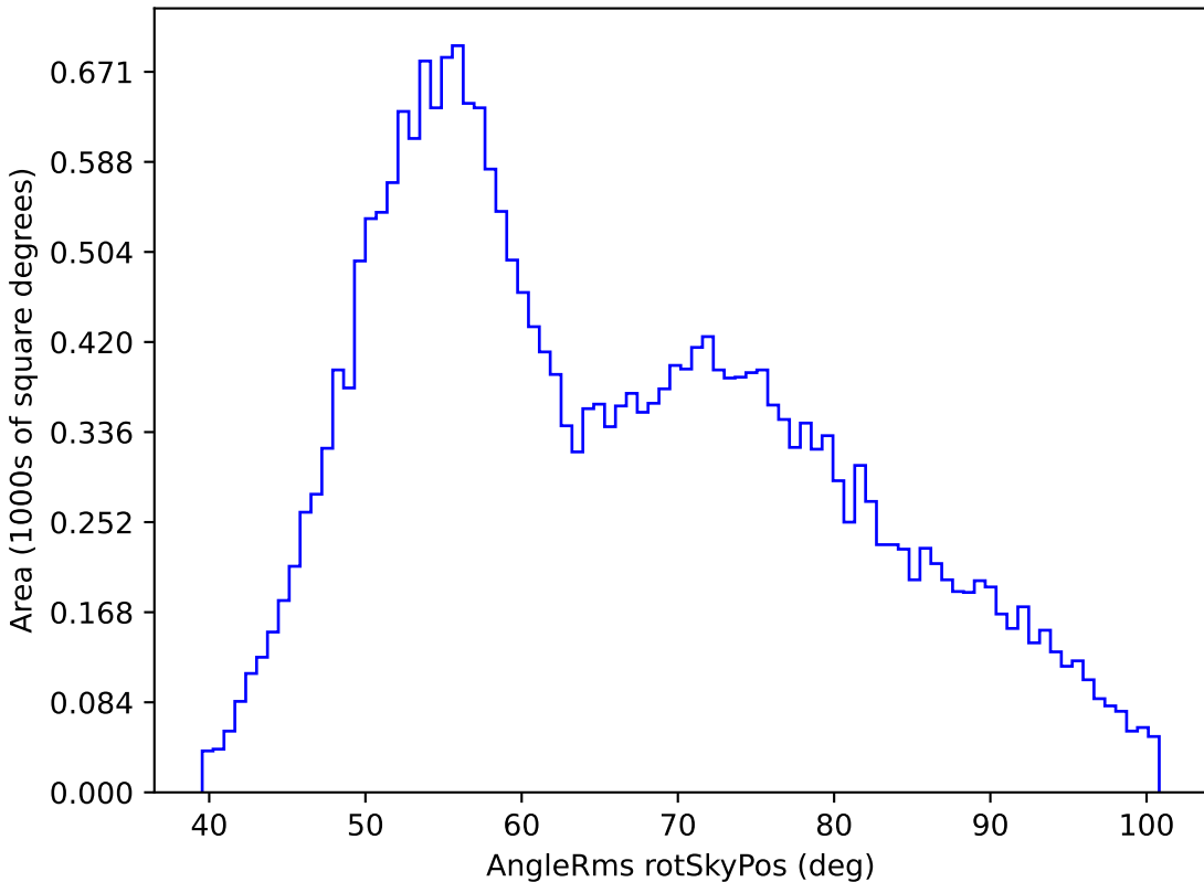
too_100_1v3.4_10yrs All sky g band: AngleRms rotSkyPos
