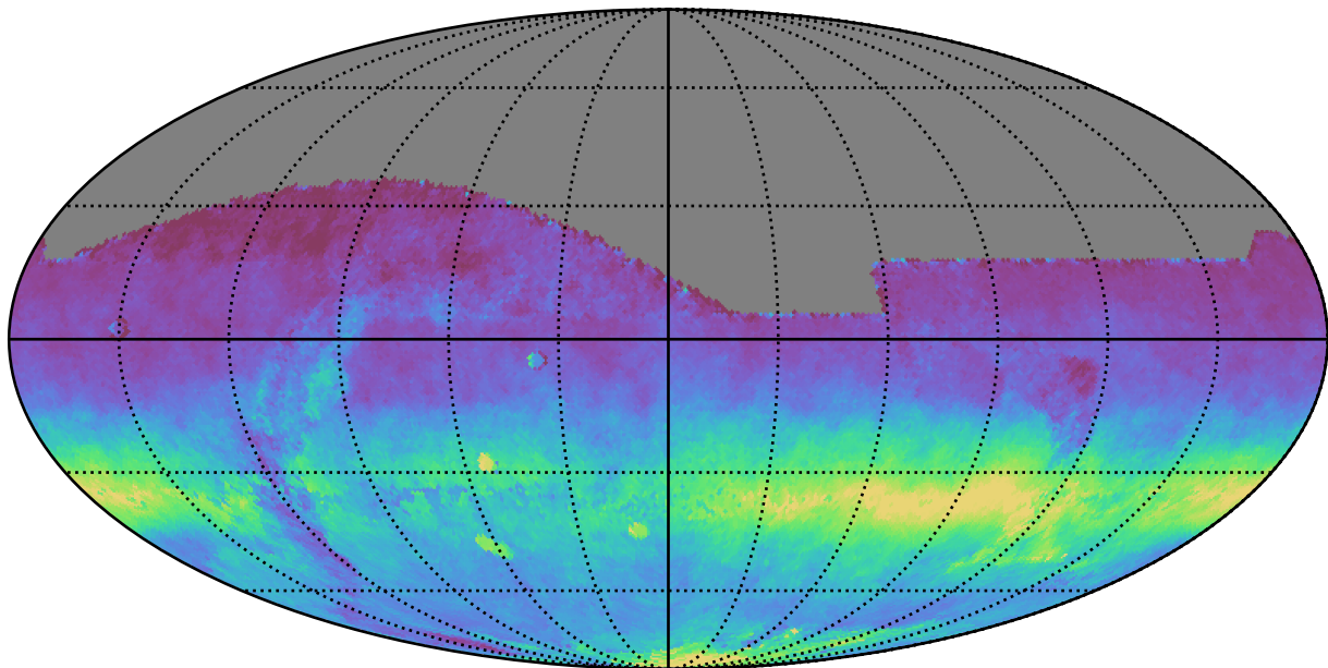
too_100_1v3.4_10yrs All sky all bands: AngleRms rotSkyPos
