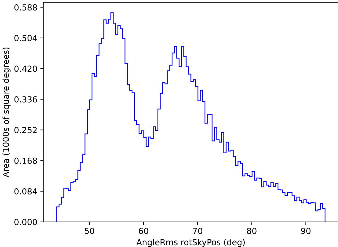
too_100_1v3.4_10yrs All sky all bands: AngleRms rotSkyPos
