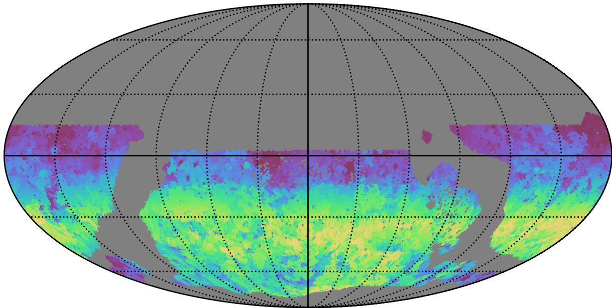
too_100_1v3.4_10yrs WFD u band: AngleRange rotSkyPos
