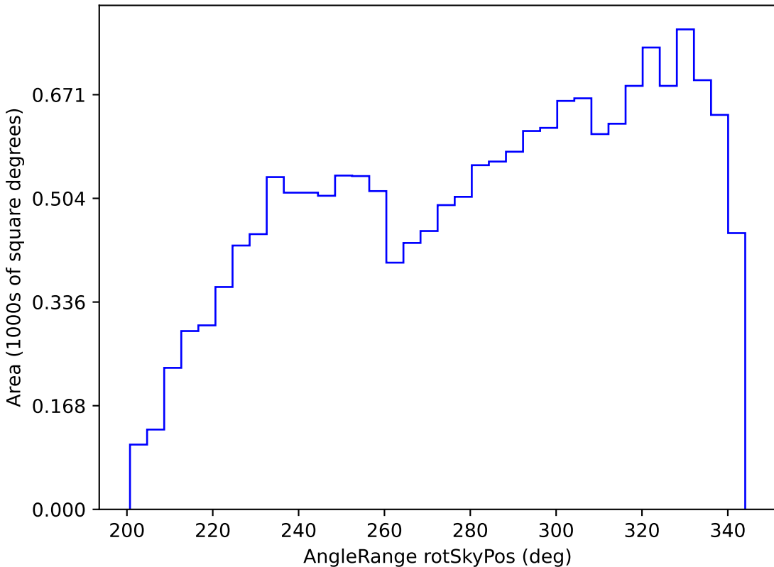
too_100_1v3.4_10yrs WFD r band: AngleRange rotSkyPos
