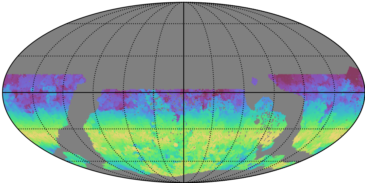
too_100_1v3.4_10yrs WFD g band: AngleRange rotSkyPos
