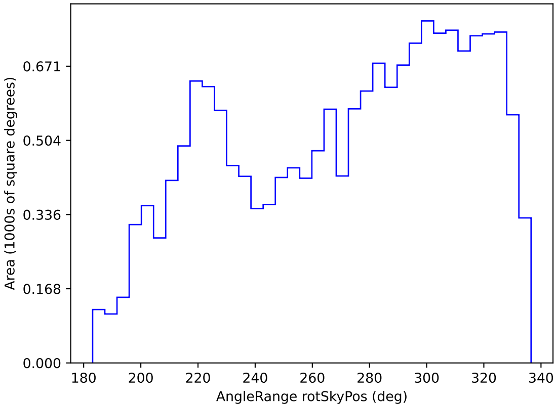
too_100_1v3.4_10yrs WFD g band: AngleRange rotSkyPos
