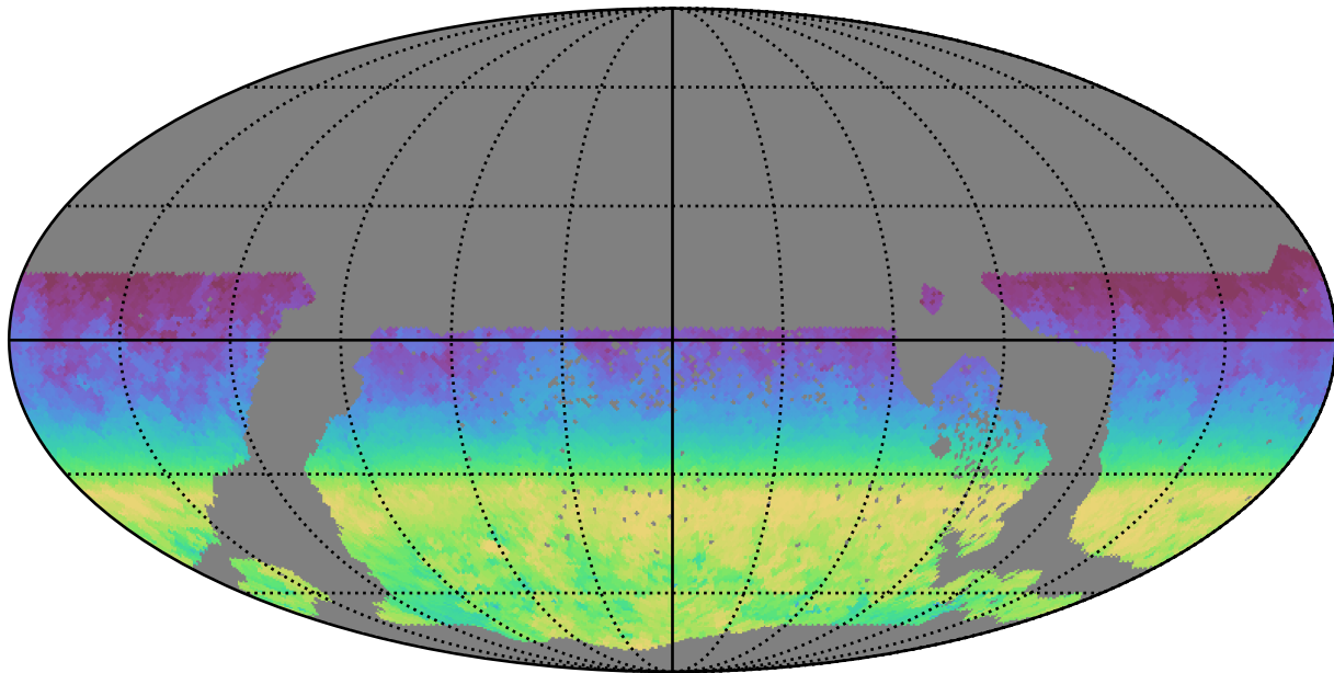
too_100_1v3.4_10yrs WFD all bands: AngleRange rotSkyPos
