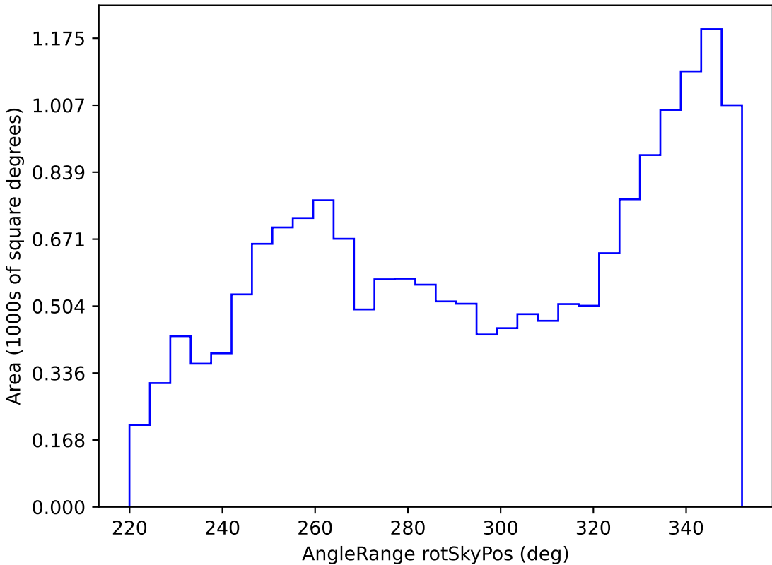
too_100_1v3.4_10yrs WFD all bands: AngleRange rotSkyPos
