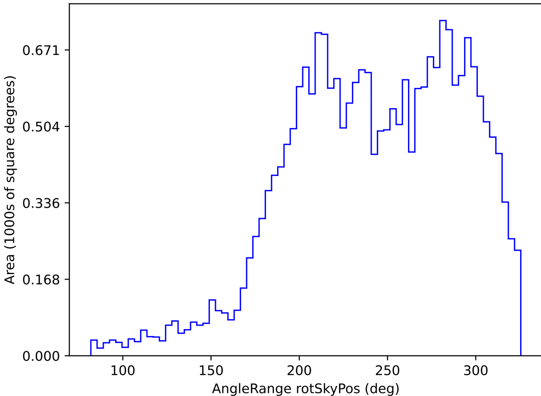
too_100_1v3.4_10yrs All sky u band: AngleRange rotSkyPos
