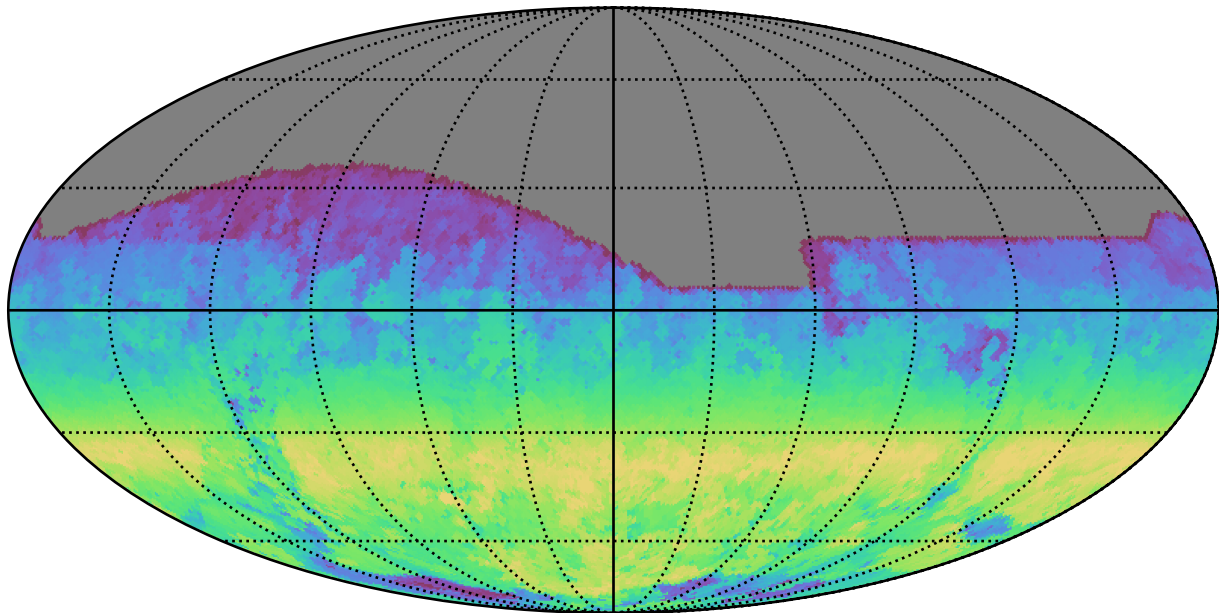
too_100_1v3.4_10yrs All sky r band: AngleRange rotSkyPos
