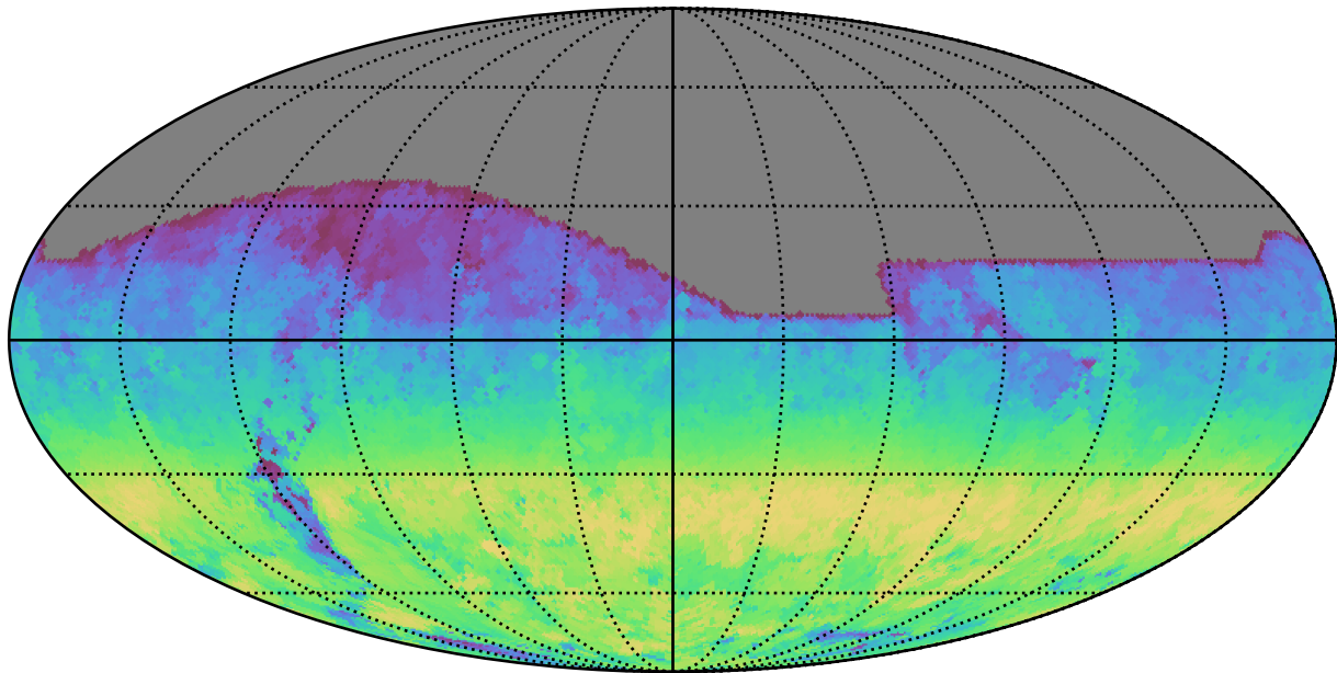
too_100_1v3.4_10yrs All sky i band: AngleRange rotSkyPos
