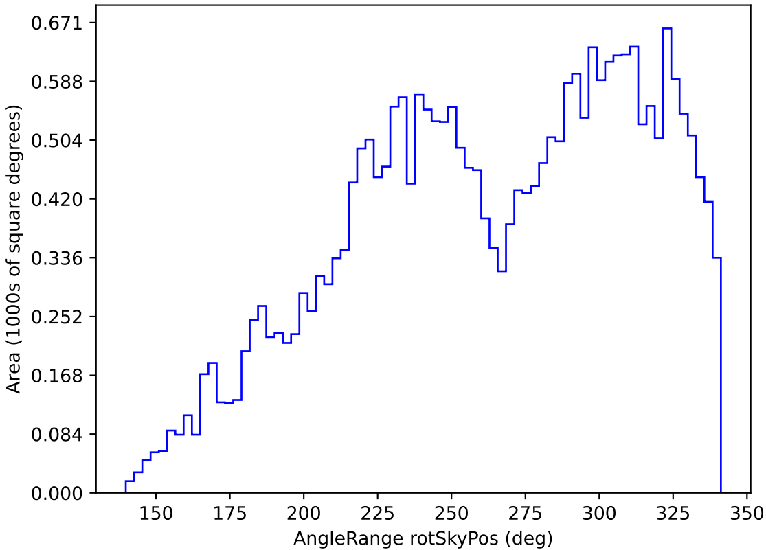
too_100_1v3.4_10yrs All sky i band: AngleRange rotSkyPos
