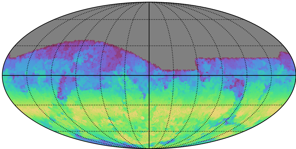
too_100_1v3.4_10yrs All sky g band: AngleRange rotSkyPos
