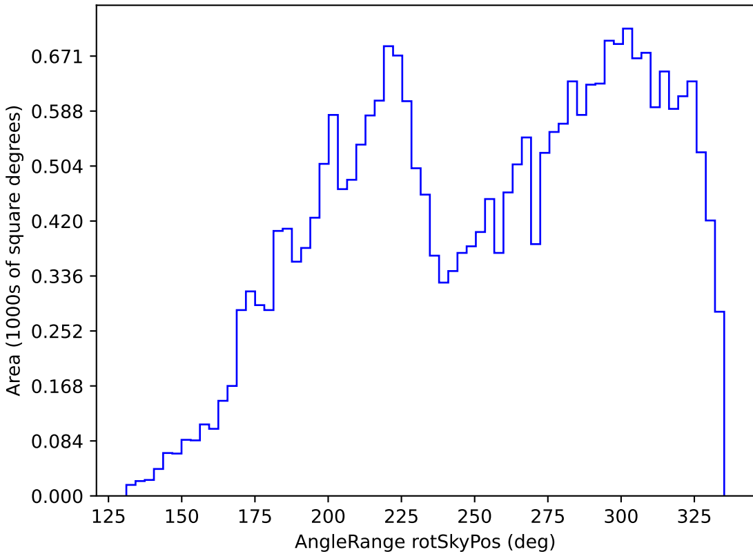
too_100_1v3.4_10yrs All sky g band: AngleRange rotSkyPos
