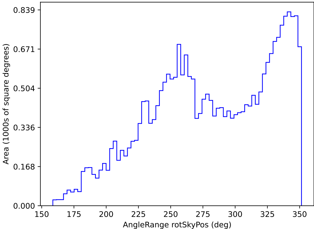
too_100_1v3.4_10yrs All sky all bands: AngleRange rotSkyPos
