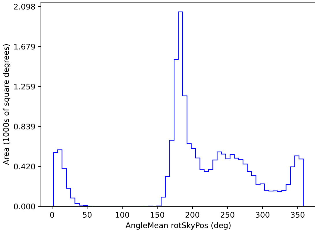
too_100_1v3.4_10yrs WFD z band: AngleMean rotSkyPos
