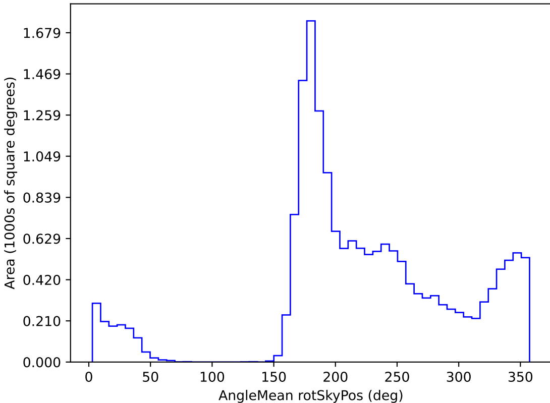
too_100_1v3.4_10yrs WFD u band: AngleMean rotSkyPos
