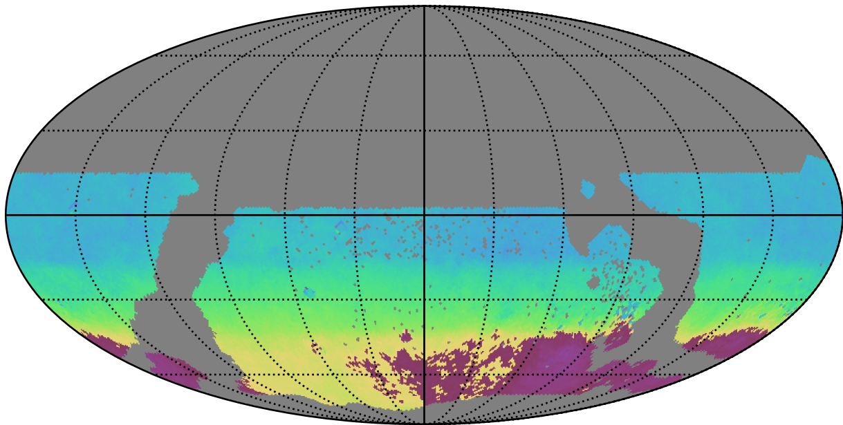
too_100_1v3.4_10yrs WFD r band: AngleMean rotSkyPos
