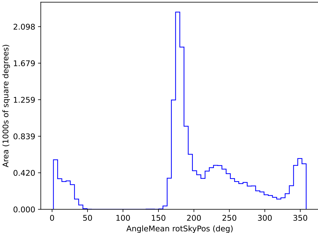
too_100_1v3.4_10yrs WFD r band: AngleMean rotSkyPos
