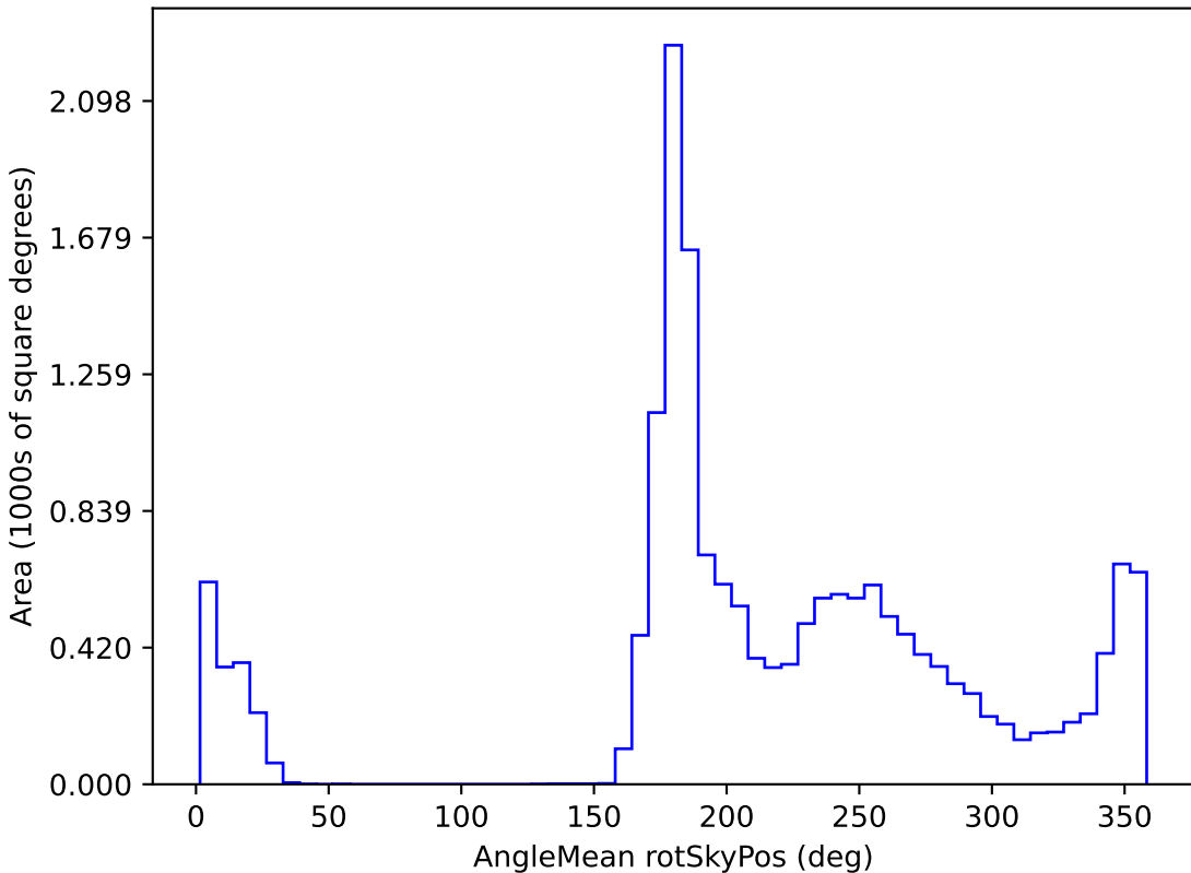
too_100_1v3.4_10yrs WFD i band: AngleMean rotSkyPos
