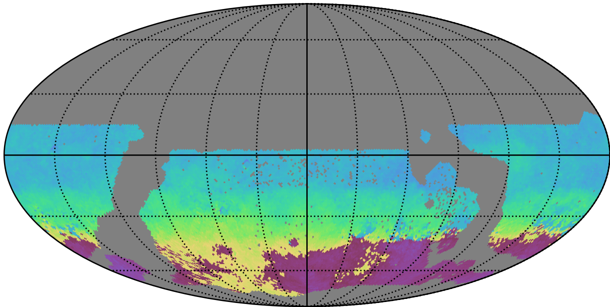
too_100_1v3.4_10yrs WFD g band: AngleMean rotSkyPos
