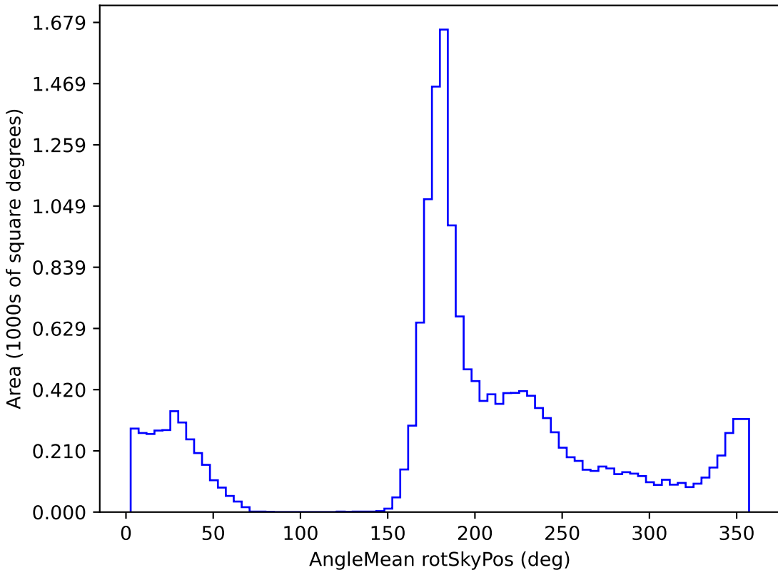
too_100_1v3.4_10yrs WFD g band: AngleMean rotSkyPos
