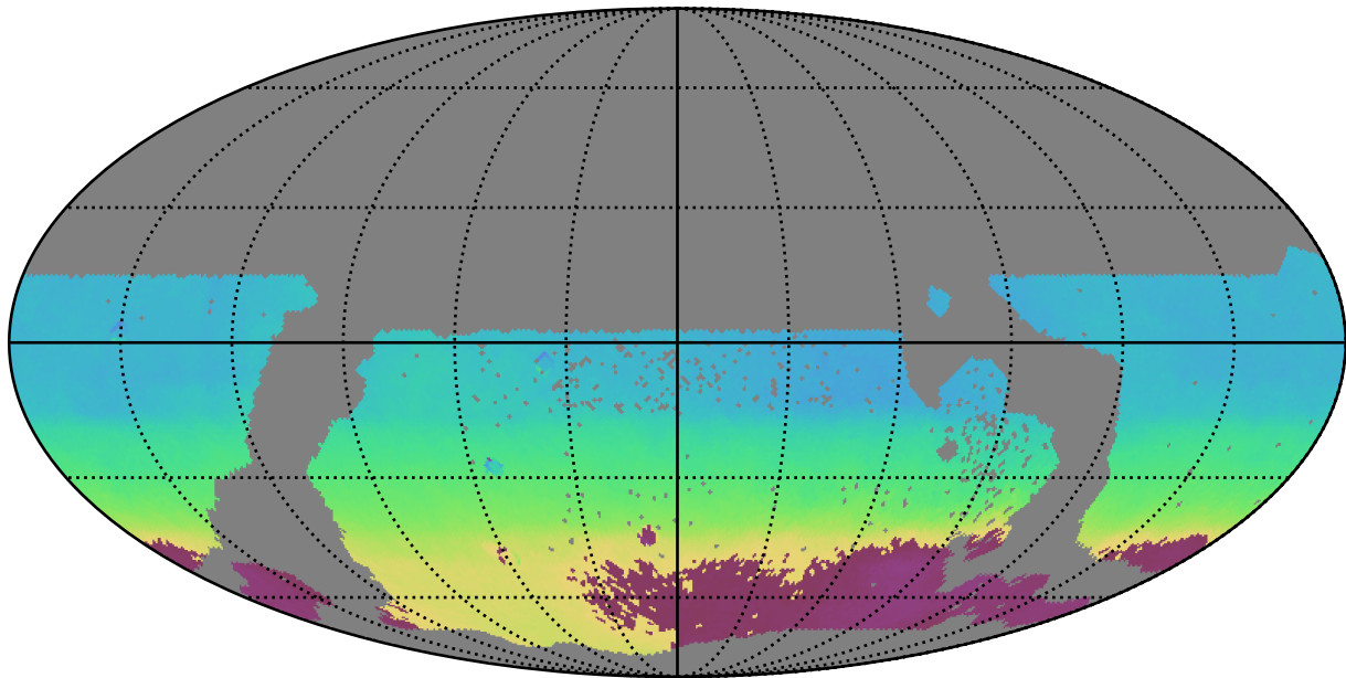
too_100_1v3.4_10yrs WFD all bands: AngleMean rotSkyPos
