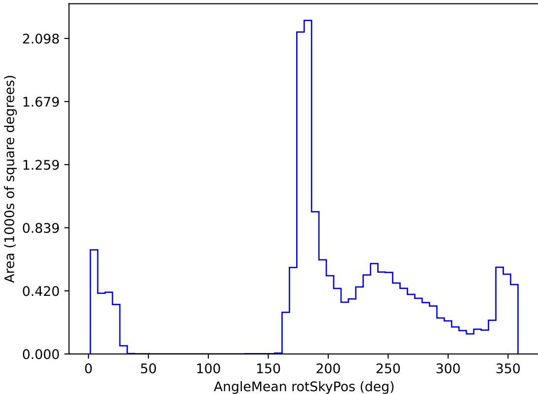
too_100_1v3.4_10yrs WFD all bands: AngleMean rotSkyPos
