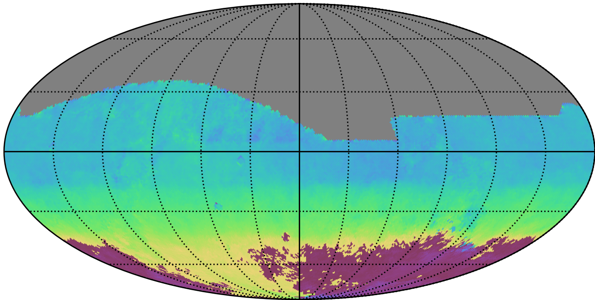
too_100_1v3.4_10yrs All sky z band: AngleMean rotSkyPos
