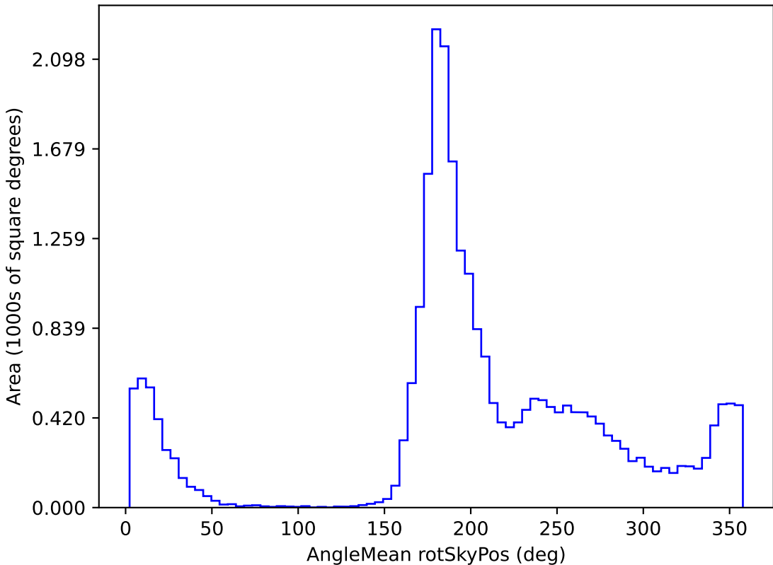
too_100_1v3.4_10yrs All sky z band: AngleMean rotSkyPos
