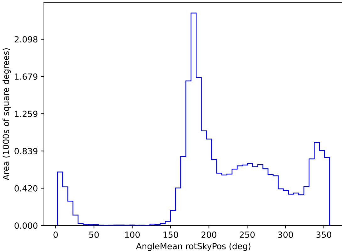
too_100_1v3.4_10yrs All sky y band: AngleMean rotSkyPos
