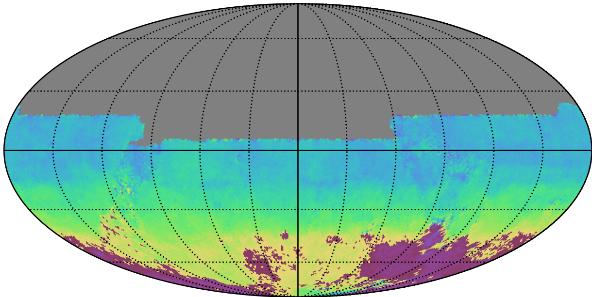
too_100_1v3.4_10yrs All sky u band: AngleMean rotSkyPos
