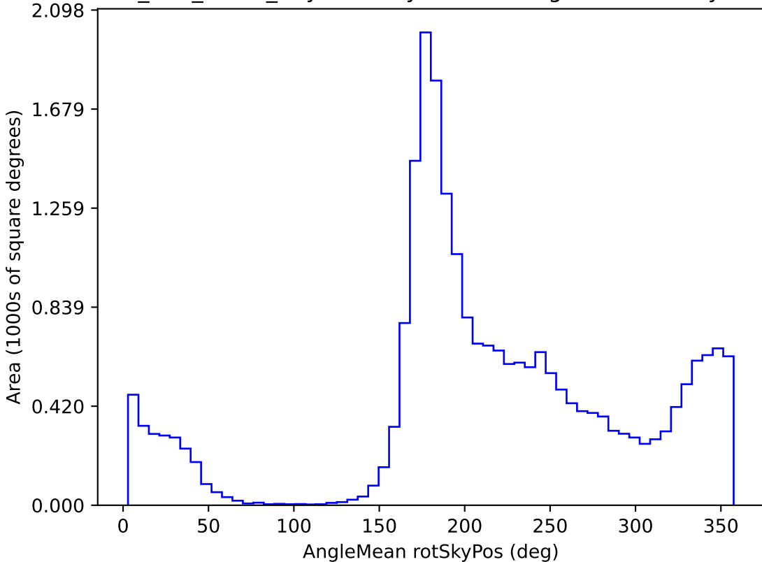
too_100_1v3.4_10yrs All sky u band: AngleMean rotSkyPos
