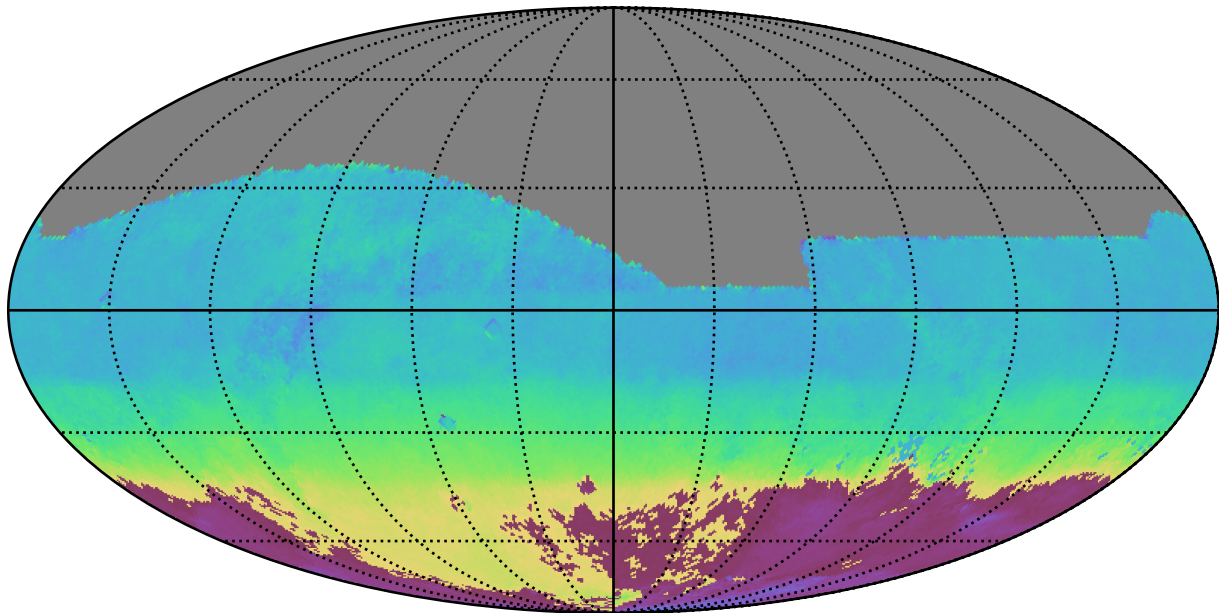
too_100_1v3.4_10yrs All sky r band: AngleMean rotSkyPos
