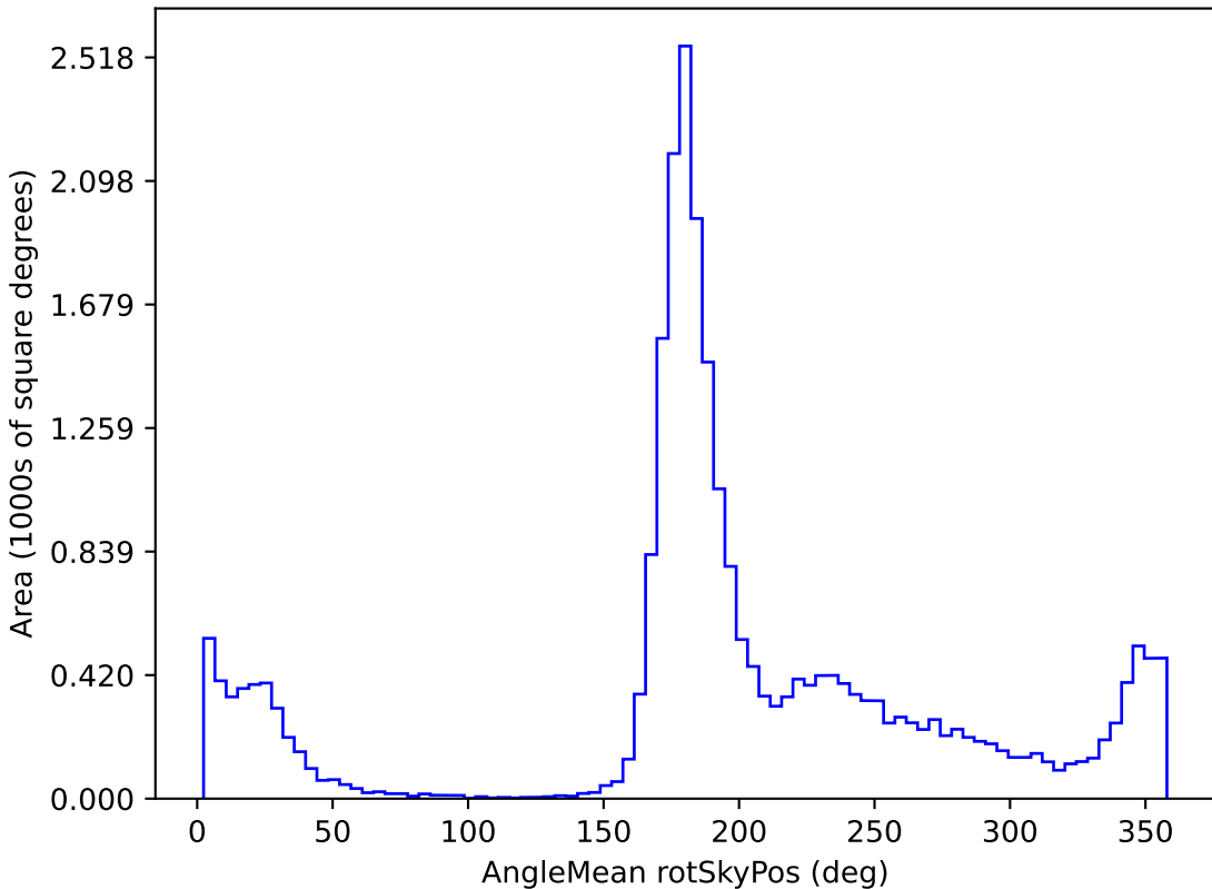
too_100_1v3.4_10yrs All sky r band: AngleMean rotSkyPos
