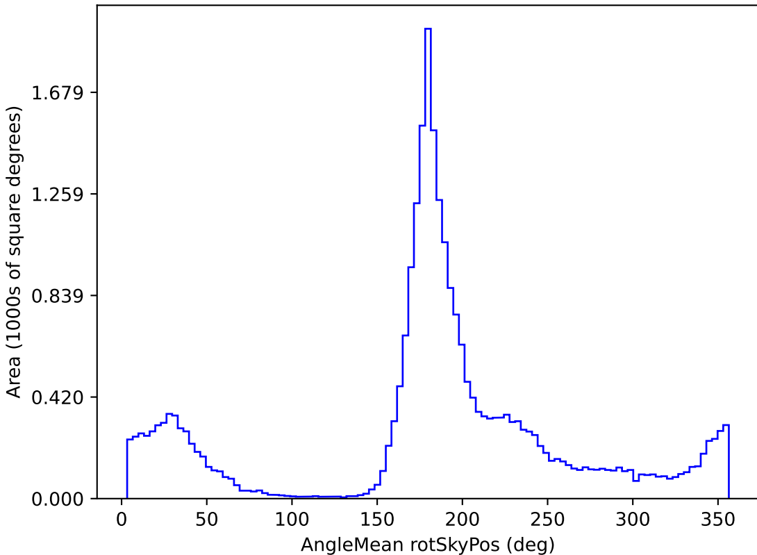
too_100_1v3.4_10yrs All sky g band: AngleMean rotSkyPos
