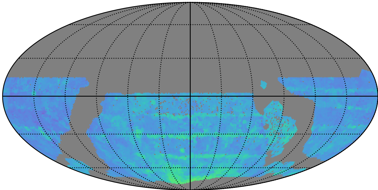
too_100_1v3.4_10yrs WFD z band: 80thPercentile Season Length
