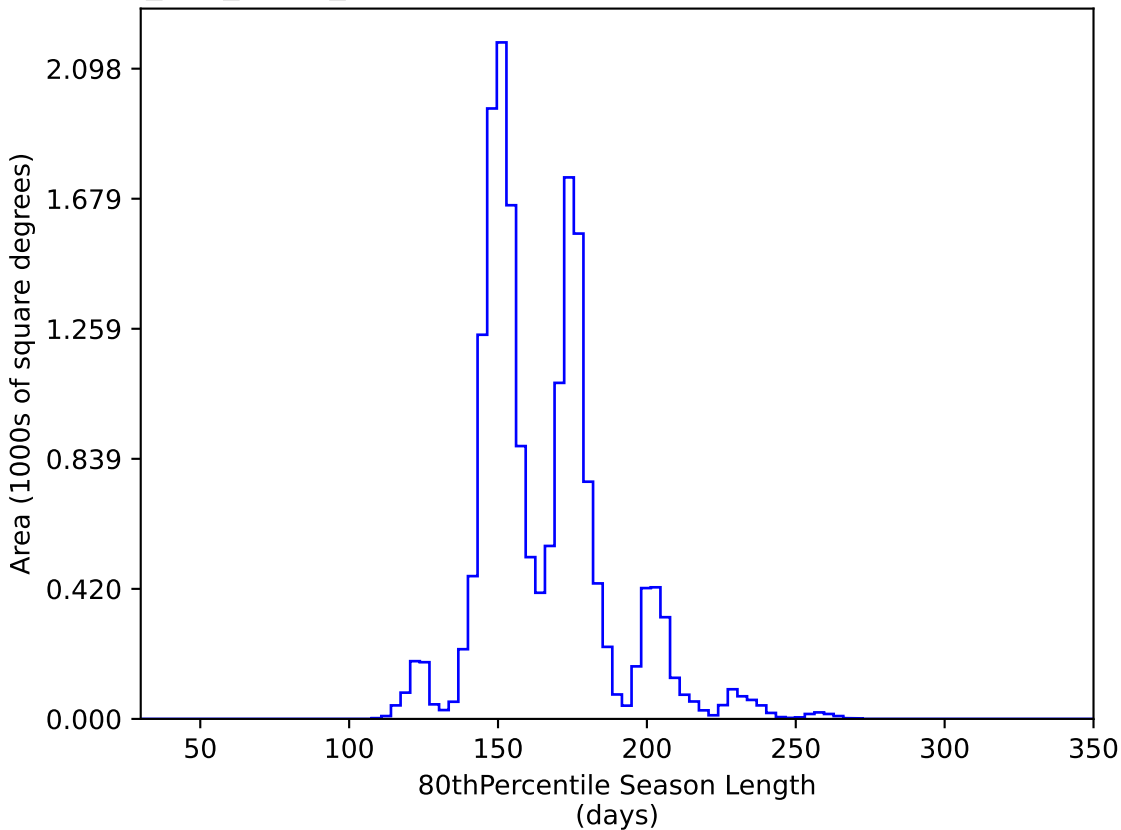
too_100_1v3.4_10yrs WFD y band: 80thPercentile Season Length
