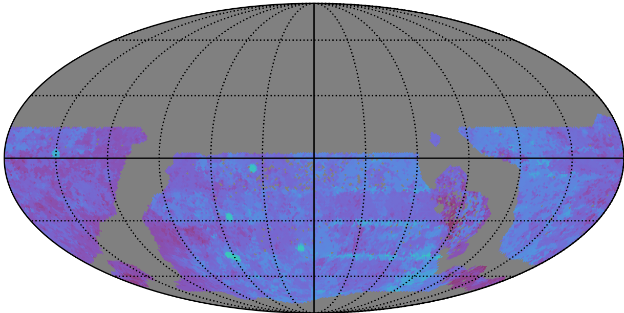
too_100_1v3.4_10yrs WFD u band: 80thPercentile Season Length
