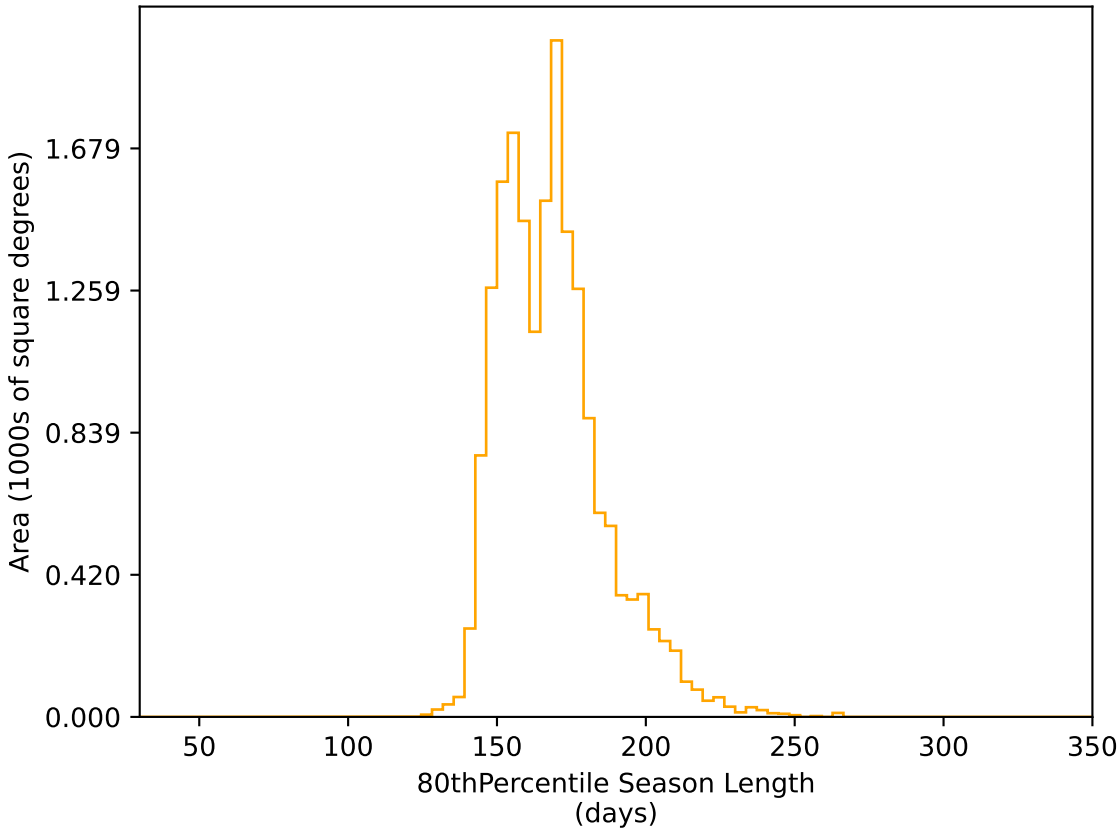
too_100_1v3.4_10yrs WFD r band: 80thPercentile Season Length
