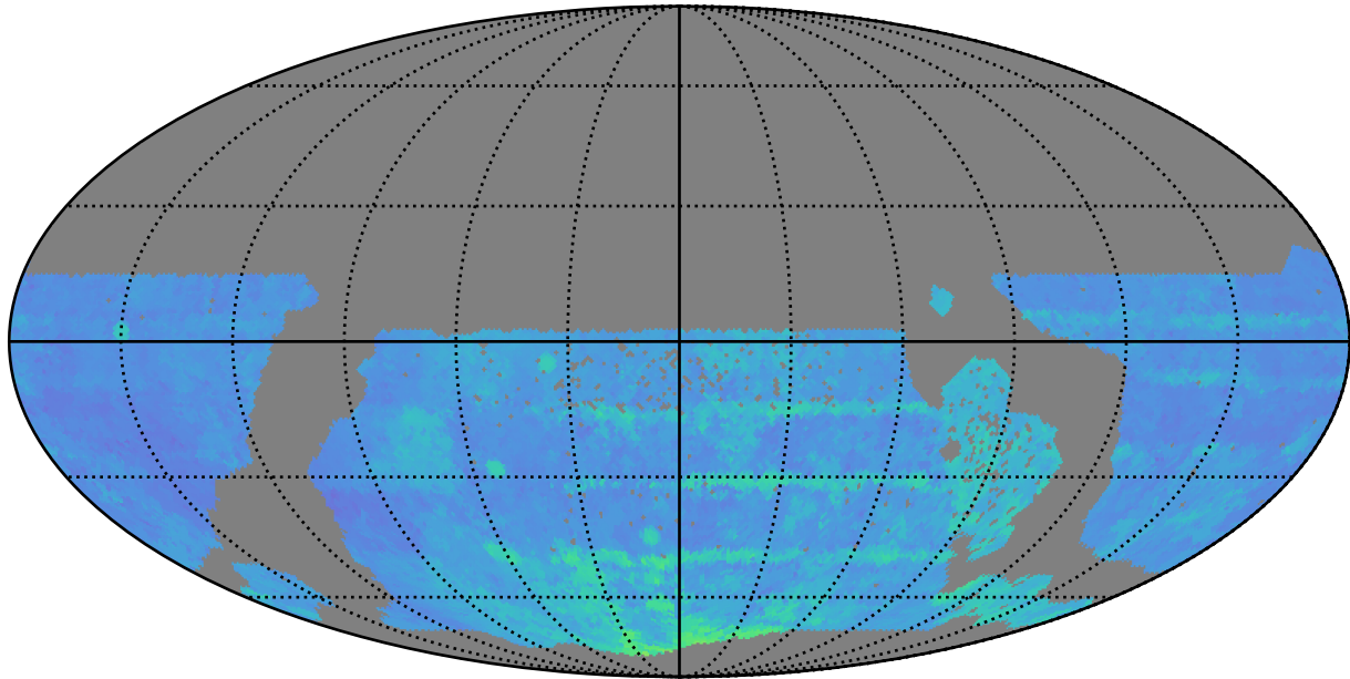
too_100_1v3.4_10yrs WFD i band: 80thPercentile Season Length
