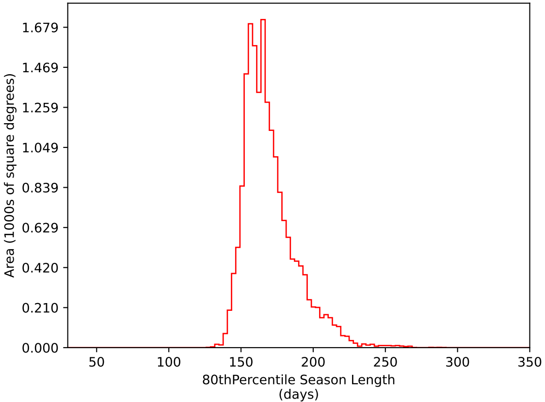
too_100_1v3.4_10yrs WFD i band: 80thPercentile Season Length
