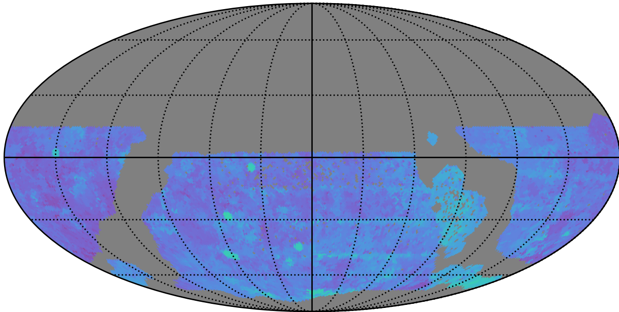
too_100_1v3.4_10yrs WFD g band: 80thPercentile Season Length
