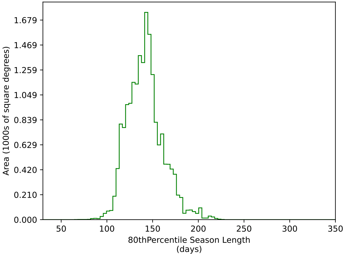
too_100_1v3.4_10yrs WFD g band: 80thPercentile Season Length
