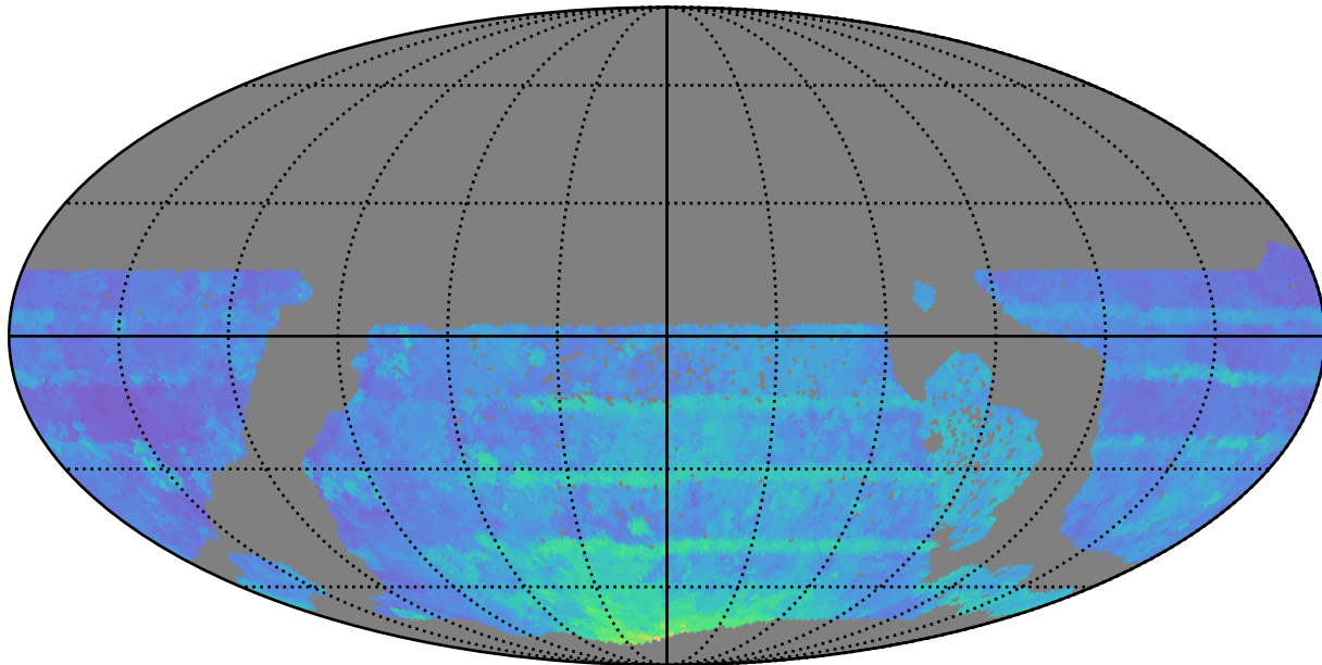
too_100_1v3.4_10yrs WFD all bands: 80thPercentile Season Length
