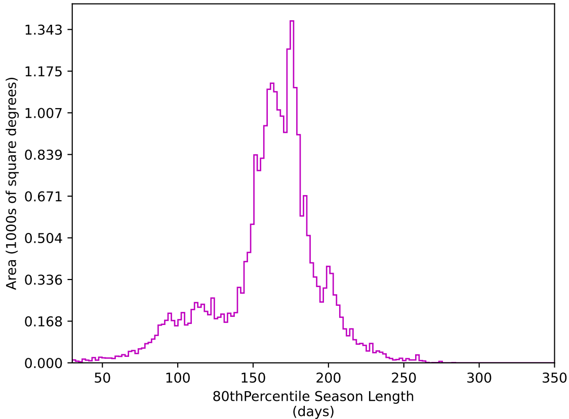
too_100_1v3.4_10yrs All sky z band: 80thPercentile Season Length
