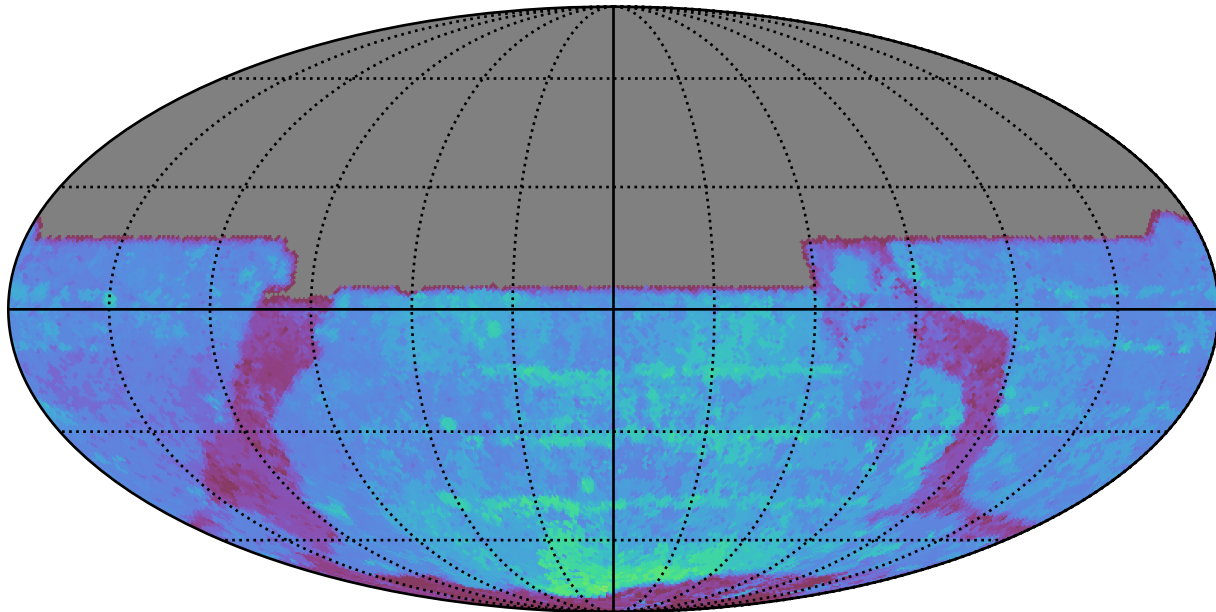
too_100_1v3.4_10yrs All sky y band: 80thPercentile Season Length
