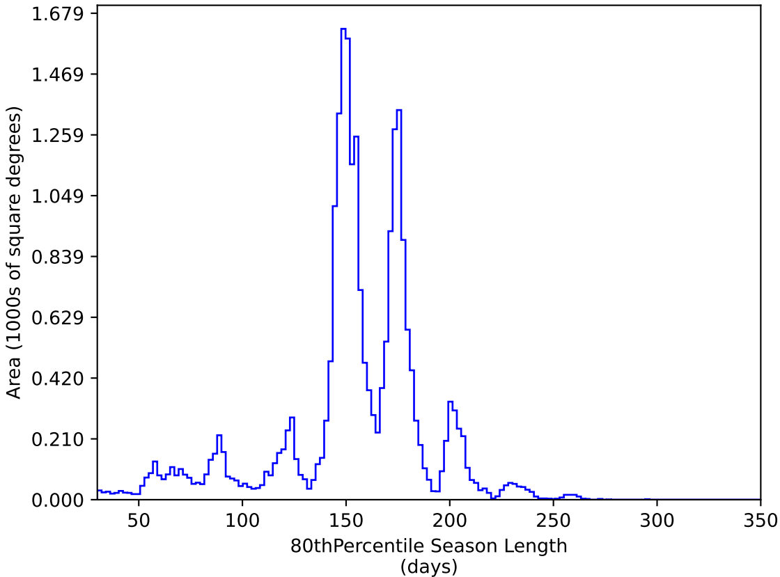
too_100_1v3.4_10yrs All sky y band: 80thPercentile Season Length
