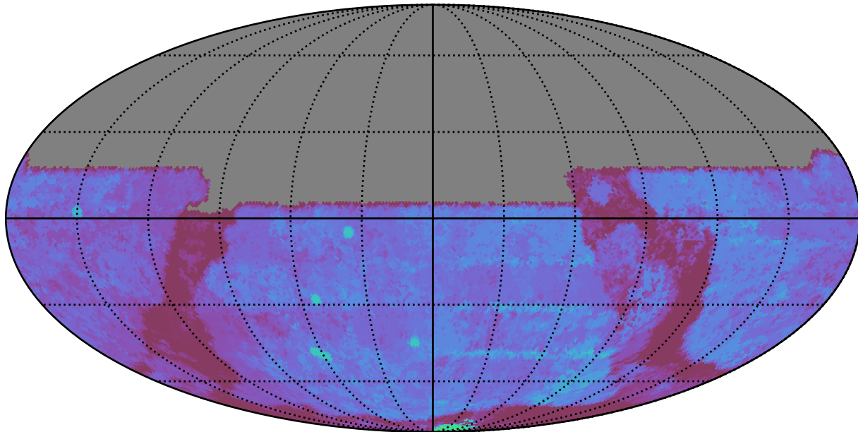
too_100_1v3.4_10yrs All sky u band: 80thPercentile Season Length
