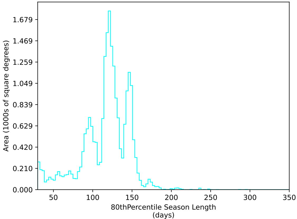
too_100_1v3.4_10yrs All sky u band: 80thPercentile Season Length
